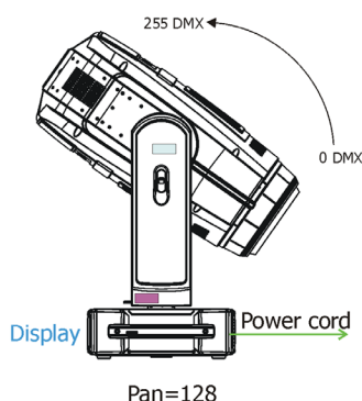
Tilt = 0 DMX
