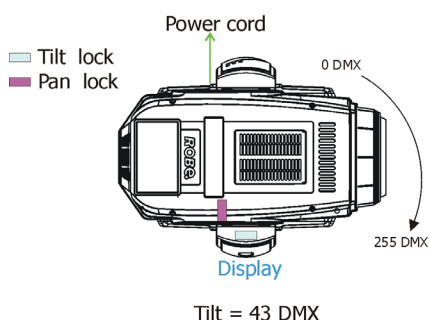
Pan = 0 DMX
