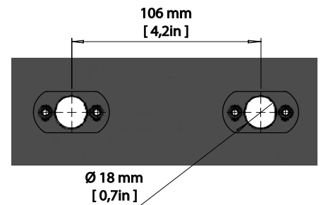
Figure 2: P-6 Series locking points
