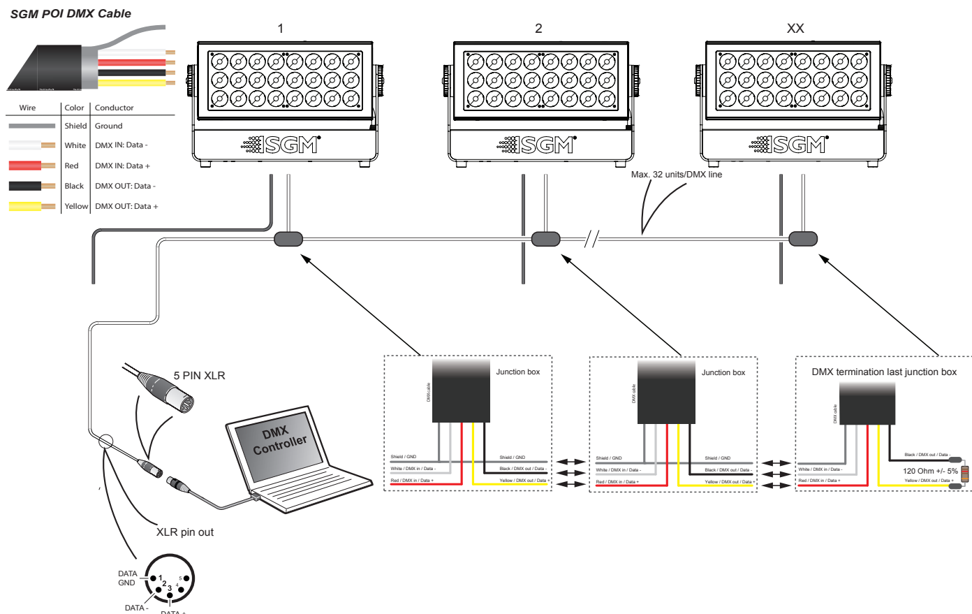
Figure 19: Connecting DMX and AC Power in P-6 POI
